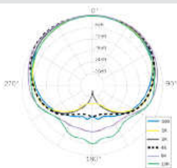
Polar Response of SR25 (typical)
