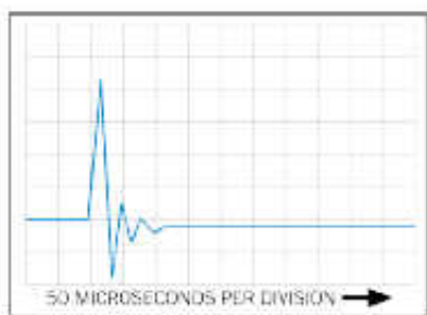
Impulse Response of SR25 (typical)
