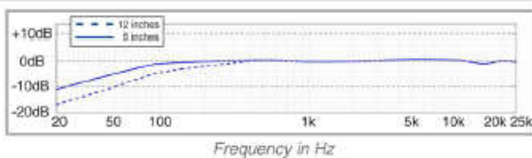
Frequency Response of SR25 (typical)
