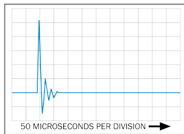
Impulse Response of SR40/HC (typical)
