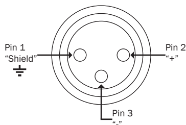
XLR Output Connector Assignment of SR40/HC
