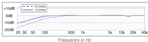
Frequency Response of SR40/HC (typical)
