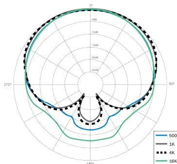
Polar Response of SR40/HC (typical)
