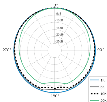
Polar Response of QTC50 (typical)
