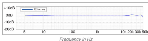
Frequency Response of QTC50 (typical)
