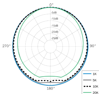
Polar Response of QTC40 (typical)
