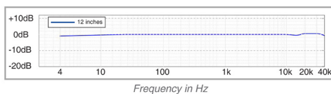
Frequency Response of QTC40 (typical)
