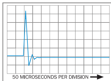
Impulse Response of QTC40 (typical)
