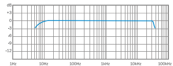
Frequency Response of QTC30 (typical)
