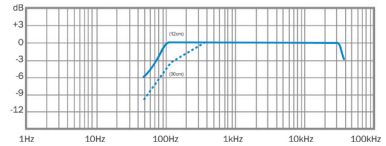
Frequency Response of P30/HC (typical)
