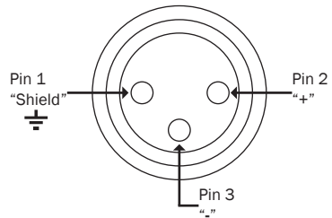
XLR Output Connector Assignment of P30/HC
