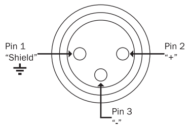
XLR Output Connector Assignment of M30BX
