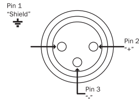
XLR Output Connector Assignment of TC25
