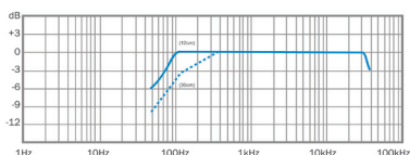
Frequency Response of SR30 (typical)
