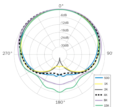
Polar Response of SR30 (typical)
